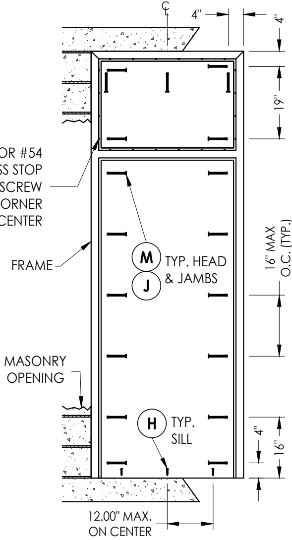
FRAME ANCHORING
